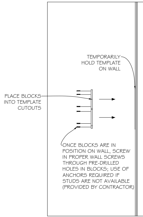
RIGHT VIEW
